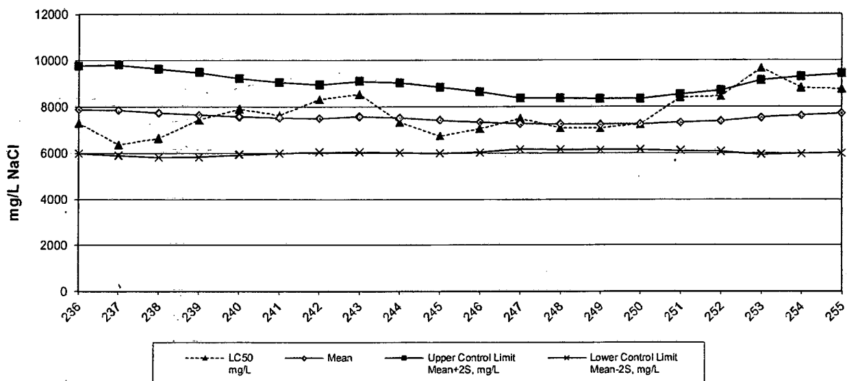
Pimephales promelas Acute Control Chart
